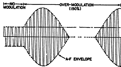
Overmodulation.
